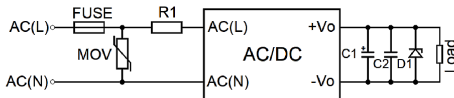
Application circuit (Figure 1)
