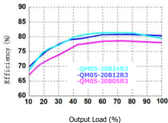
Efficiency VS out load (Vin=230VAC)
