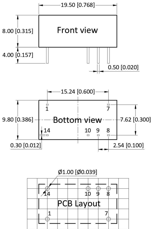
Figure 7: Overall dimensions
