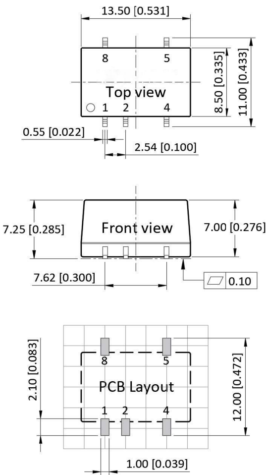
Figure 7: Overall dimensions
