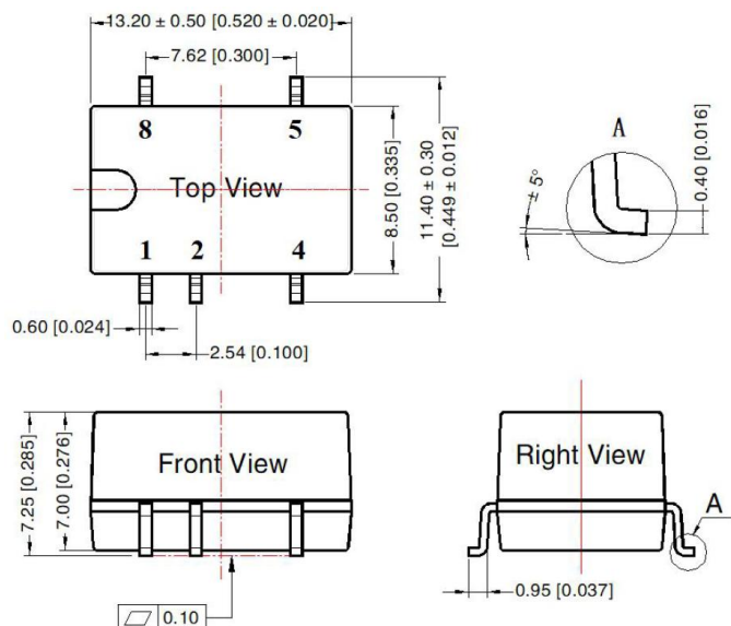
Figure 7: Overall dimensions
