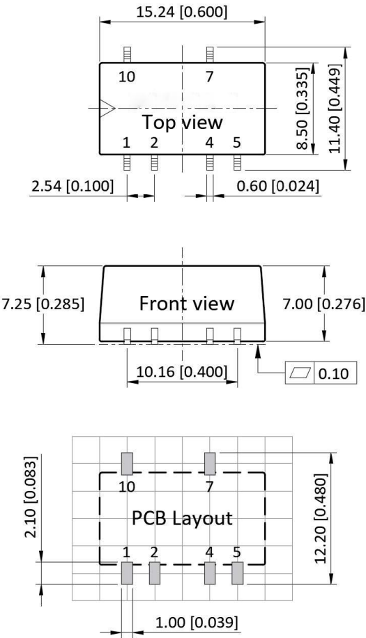
Figure 7: Overall dimensions
