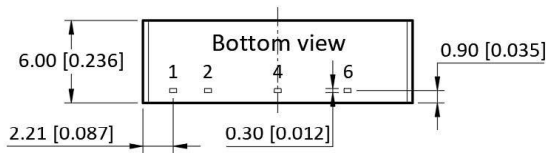
Figure 7: Overall dimensions
