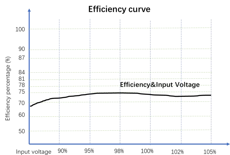
Figure 6: Efficiency VS Input Voltage (100% Load)
