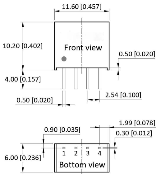
Figure 7: Overall dimensions
