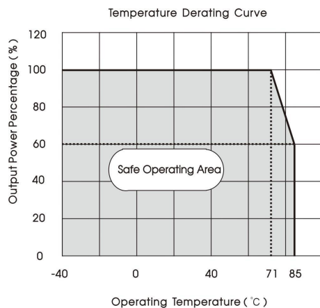
Fig.1 K78UXX-500R3 K78U24-300R3 (Vin=36V~60V)
