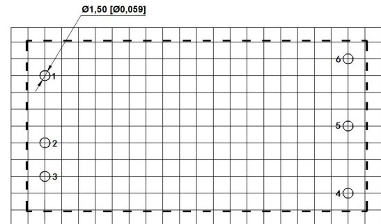
PCB Printing Layout &amp; Pin Definition Table
