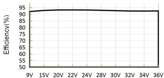
Efficiency VS input voltage (full load) (2405LD)
