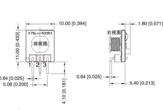
Figure 7: Overall dimensions
