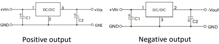
Figure 1: Application circuit
