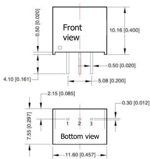
Figure 7: Overall dimensions
