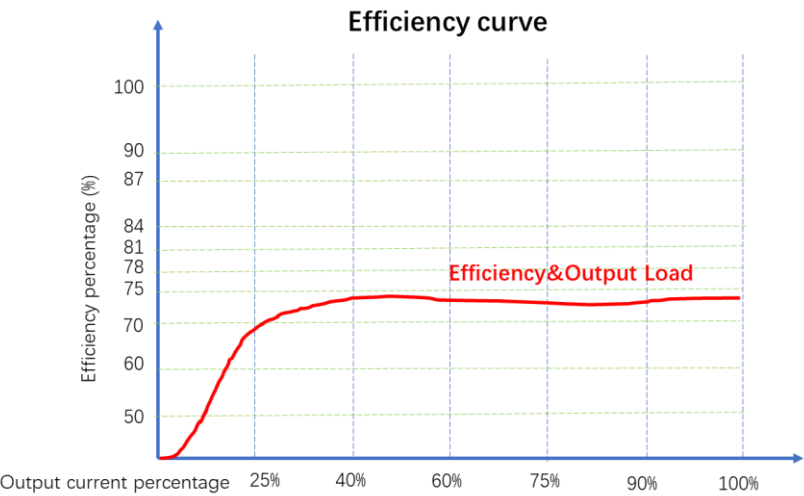
Figure 5: Efficiency VS Output Load (Nominal Voltage Input)
