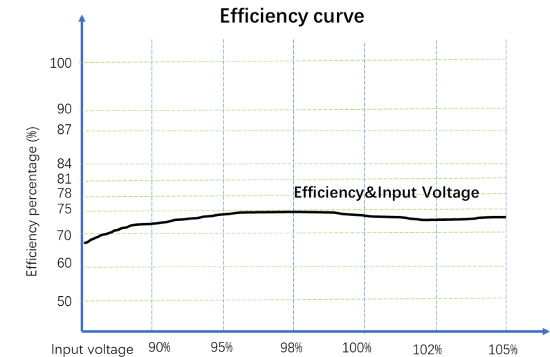
Figure 6: Efficiency VS Input Voltage (100% Load)
