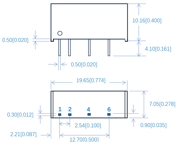
Figure 7: Overall dimensions
