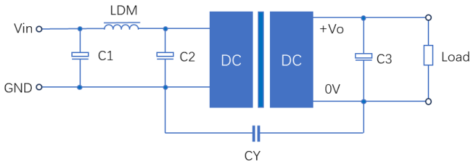
Figure 2: EMC Typical Recommended Circuits
