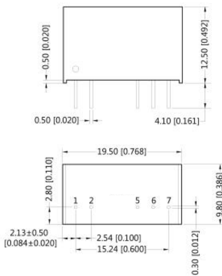
Figure 7: Overall dimensions
