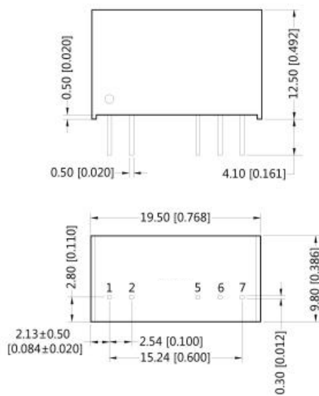
Figure 7: Overall dimensions
