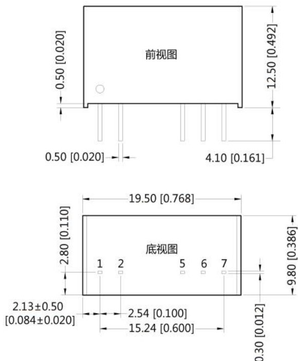
Figure 7: Overall dimensions
