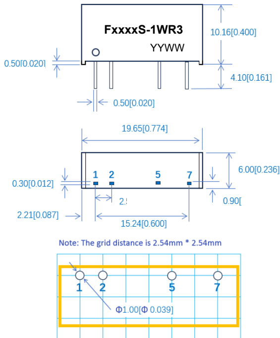
Figure 7: Overall dimensions
