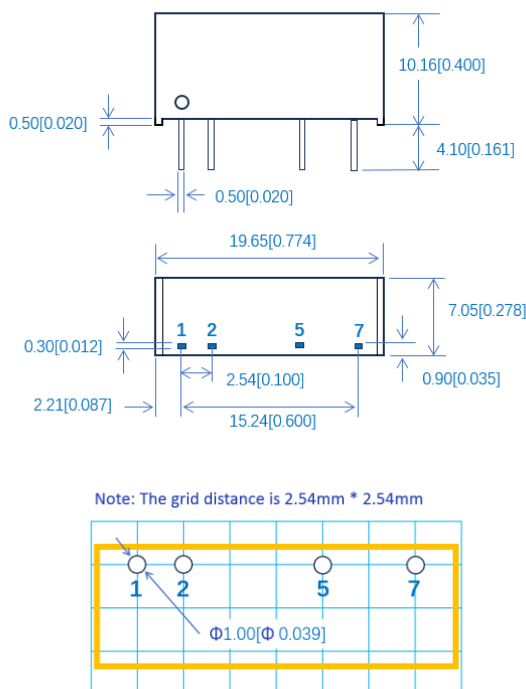
Figure 7: Overall dimensions
