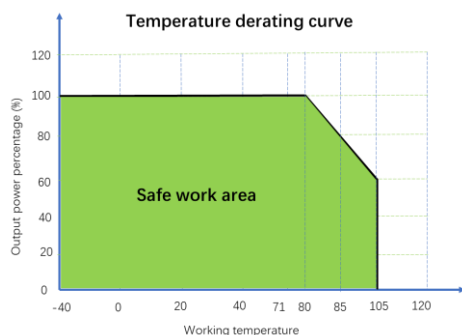
Figure 4: Temperature Derating Curve
