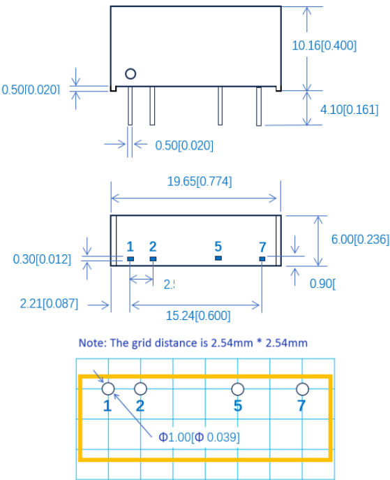
Figure 7: Overall dimensions
