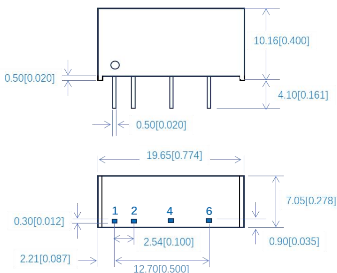
Figure 7: Overall dimensions
