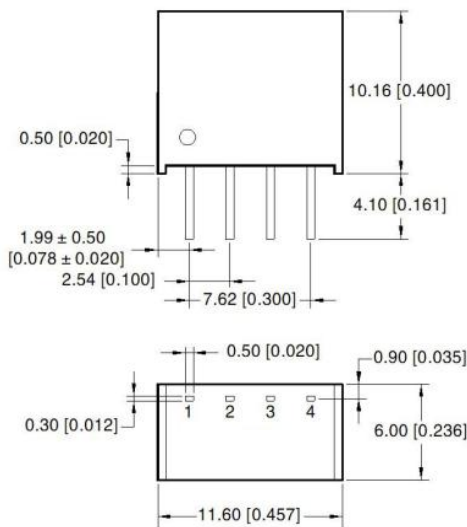
Figure 7: Overall dimensions
