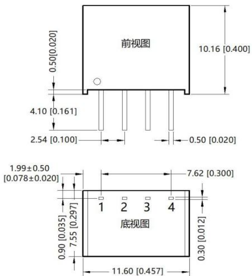
Figure 7: Overall dimensions
