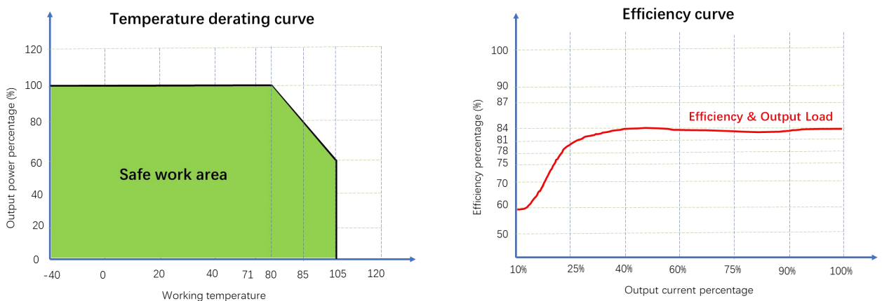
Figure 5: Efficiency VS Output Load (Nominal Voltage Input)
