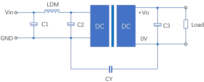
Figure 2: EMC Typical Recommended Circuits
