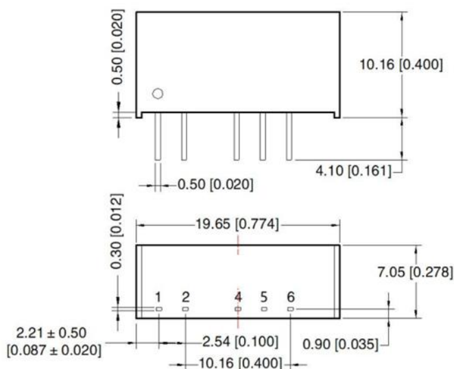
Figure 7: Overall dimensions
