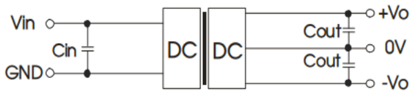
Figure 1: Application circuit
