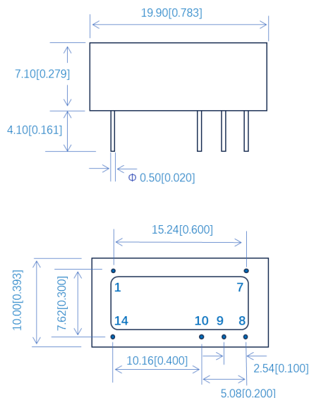
Figure 7: Overall dimensions
