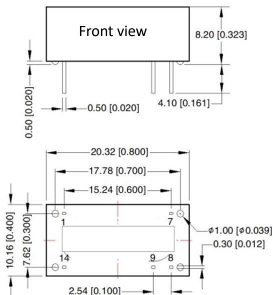
Figure 7: Overall dimensions
