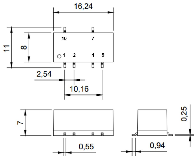
Figure 7: Overall dimensions
