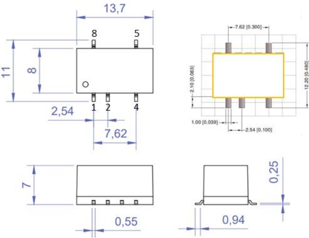
Figure 7: Overall dimensions
