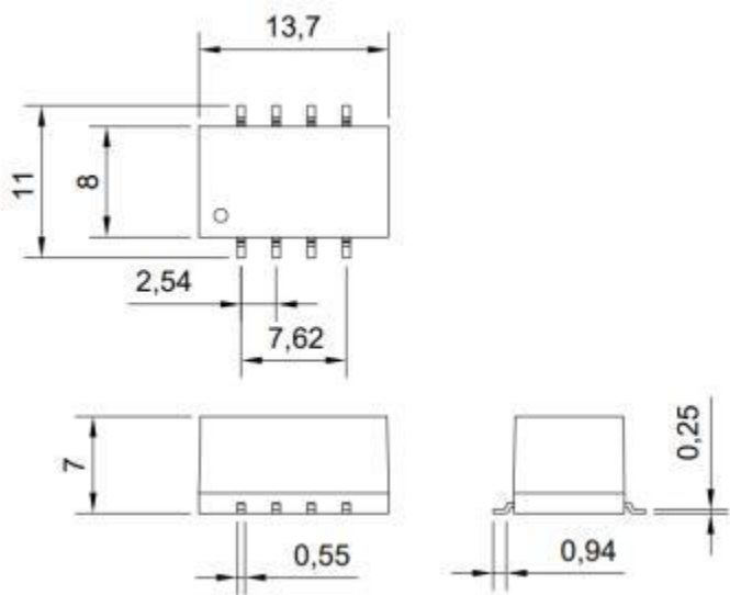
Figure 7: Overall dimensions
