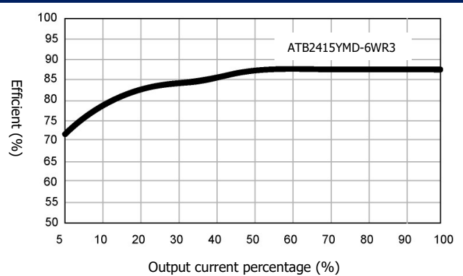
Efficiency Vs Output Voltage (Vin=24V)
