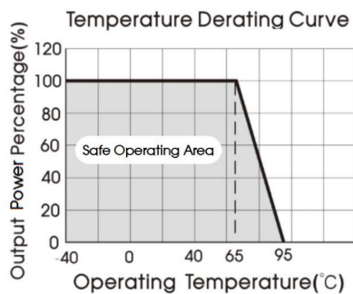
GTB24_YMD-20WR3/GTB48_YMD-20WR3 series Nominal input voltage, 3.3V, 5V output
