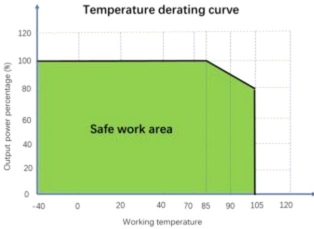
Figure 4: Temperature Derating Curve 图4: 温度减额曲线
