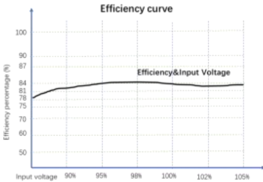
Figure 6: Efficiency VS Input Voltage (100% Load) 图6: 效率与输入电压 (100%负载)
