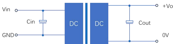
Figure 1: Application circuit
