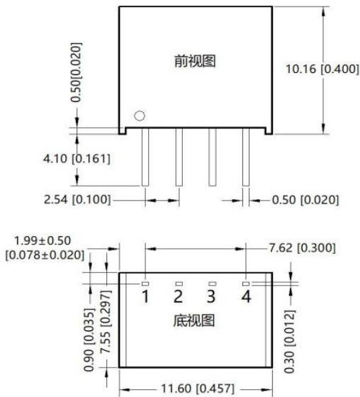
Figure 7: Overall dimensions
