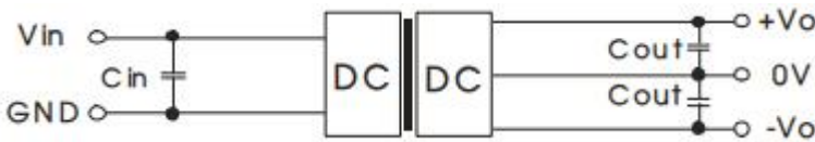
Figure 1: Application circuit
