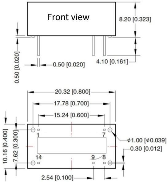
Figure 7: Overall dimensions
