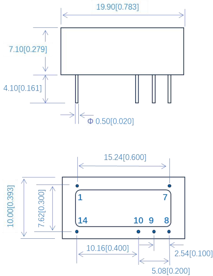
Figure 7: Overall dimensions 图7: 外形尺寸
