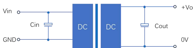
Figure 1: Application circuit
