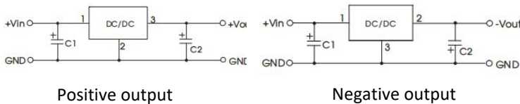
Figure 1: Application circuit
