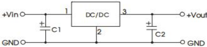
Figure 1: Application circuit
