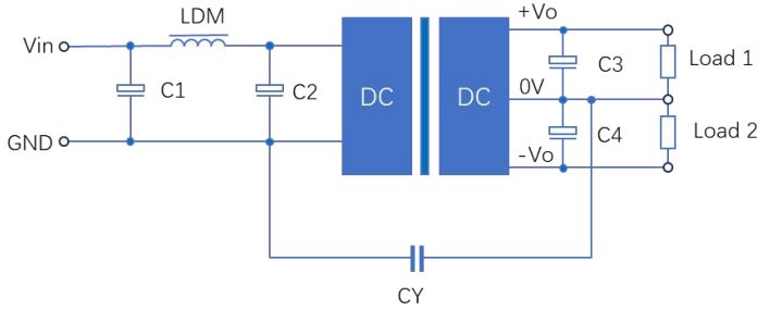
Figure 2: EMC Typical Recommended Circuits 图2:EMC典型推荐电路
