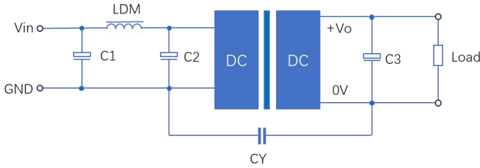
Figure 2: EMC Typical Recommended Circuits 图2:EMC典型推荐电路
