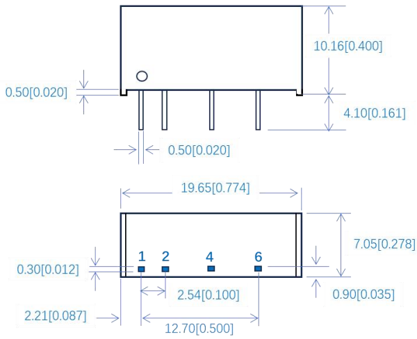
Figure 7: Overall dimensions 图7: 外形尺寸
