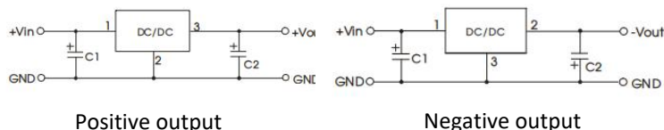
Figure 1: Application circuit
