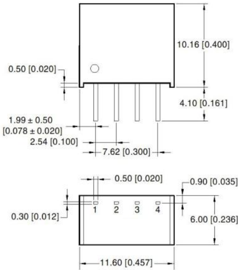
Figure 7: Overall dimensions 图7: 外形尺寸
