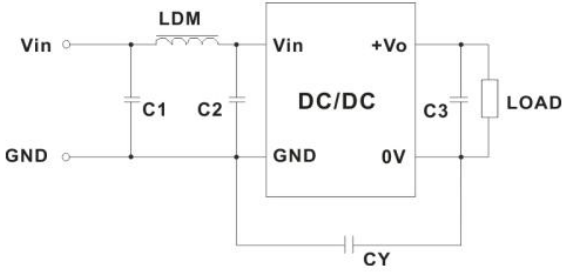
Figure 2: EMC Typical Recommended Circuits 图2:EMC典型推荐电路
