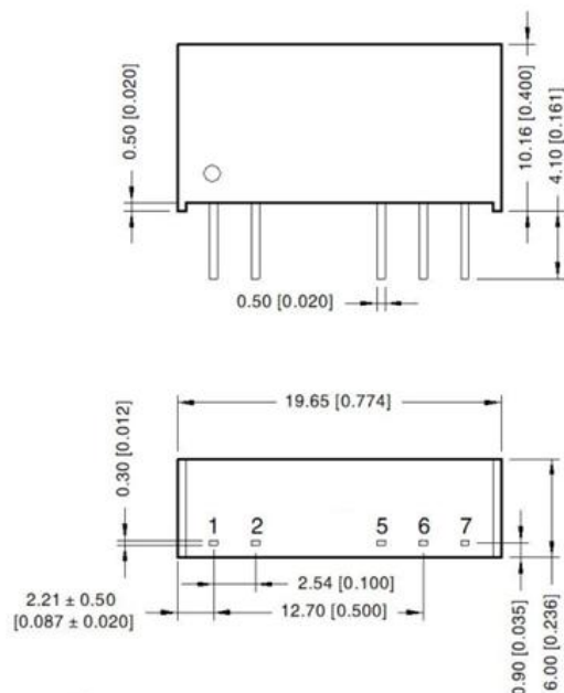
Figure 7: Overall dimensions
