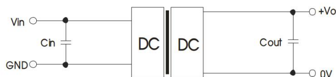
Figure 1: Application circuit
