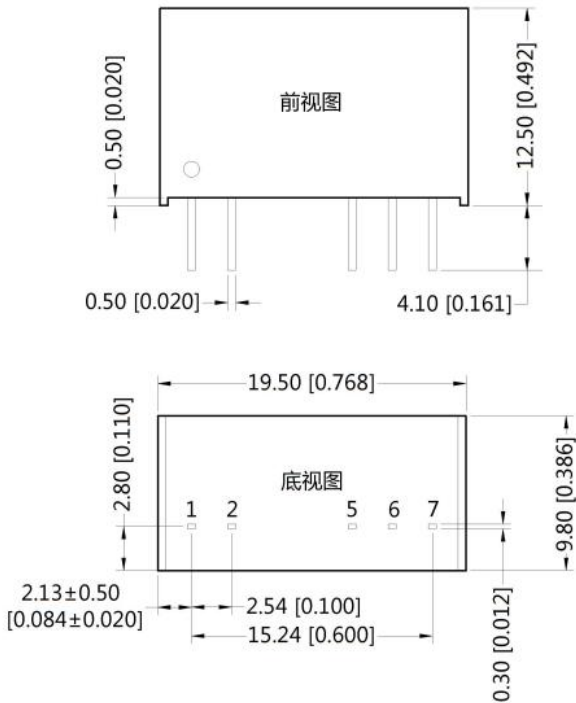
Figure 7: Overall dimensions
