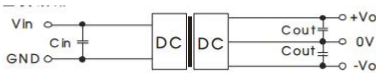
Figure 1: Application circuit
