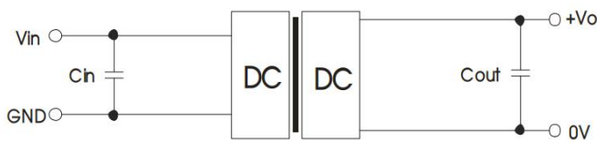
Figure 1: Application circuit
