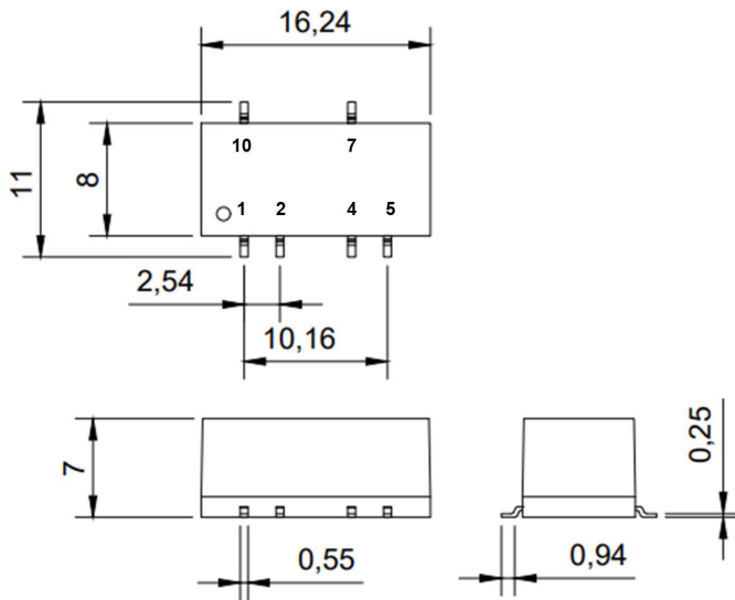
Figure 7: Overall dimensions
