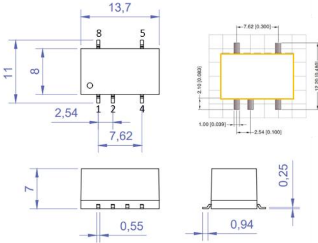
Figure 7: Overall dimensions
